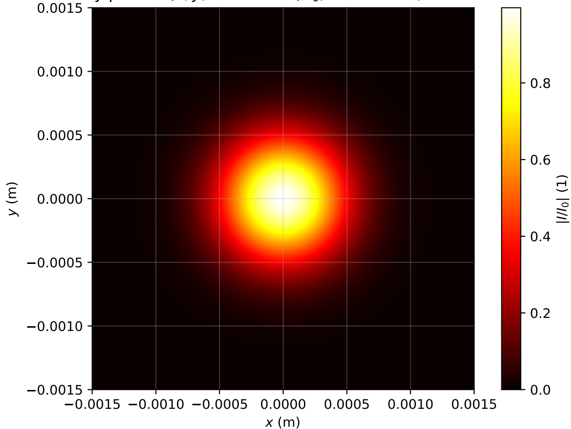
Intensity profile I(x, y, z = 0.159m)/I_0 , Pin=0.1Pcr, artificial time
